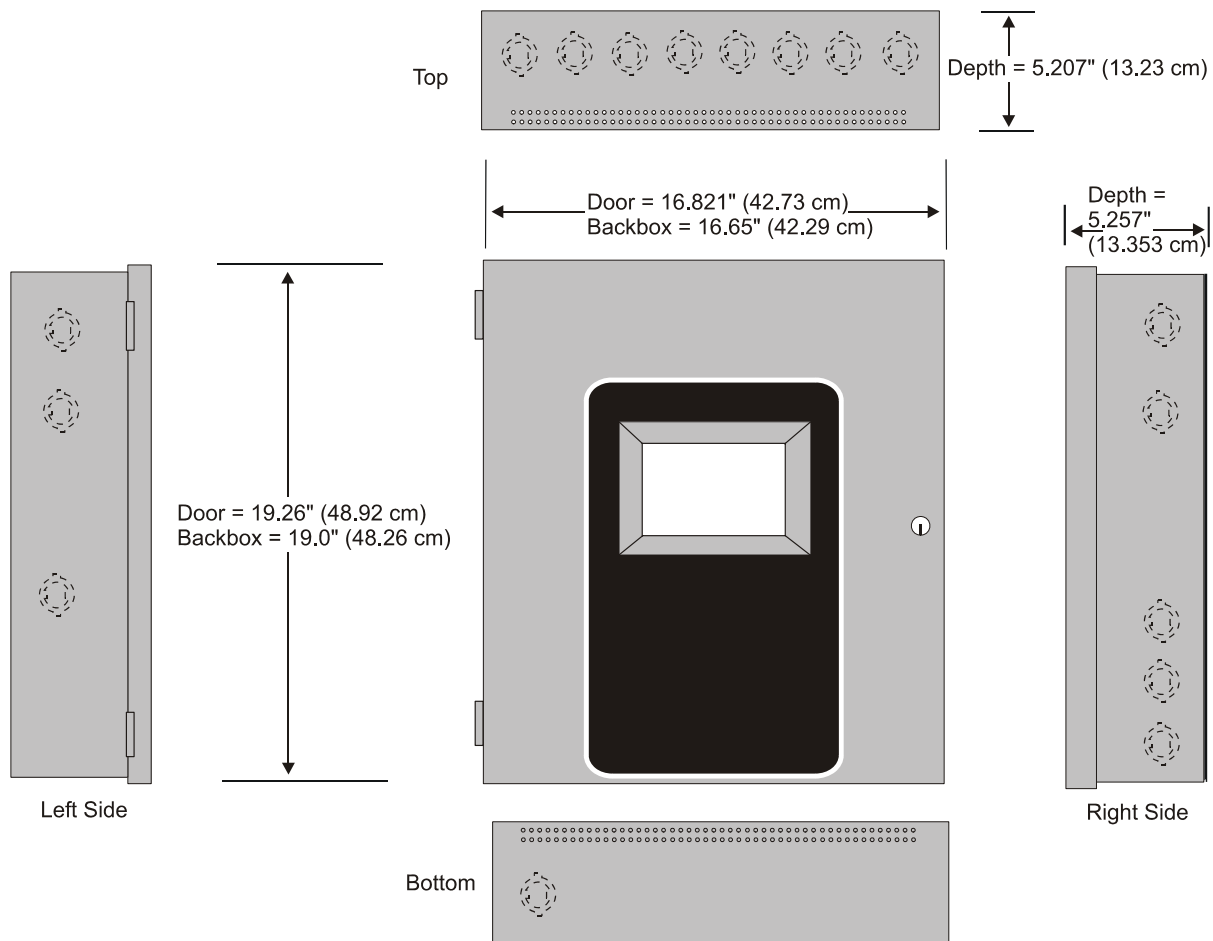
Cabinet measurements
